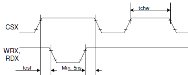
Figure 5 CSX timing
